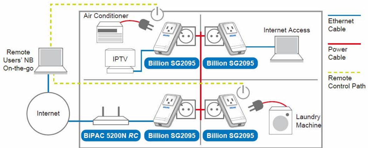
▲ The connected home using the Billion SG2095
